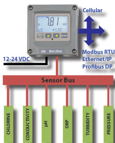
Figure 1: MetriNet system
