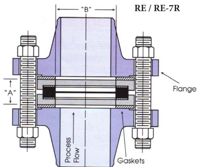
Type RE graphite rupture disk in RE-7R safety head
